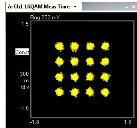
Figure 2. QAM16 at 64 GBaud
